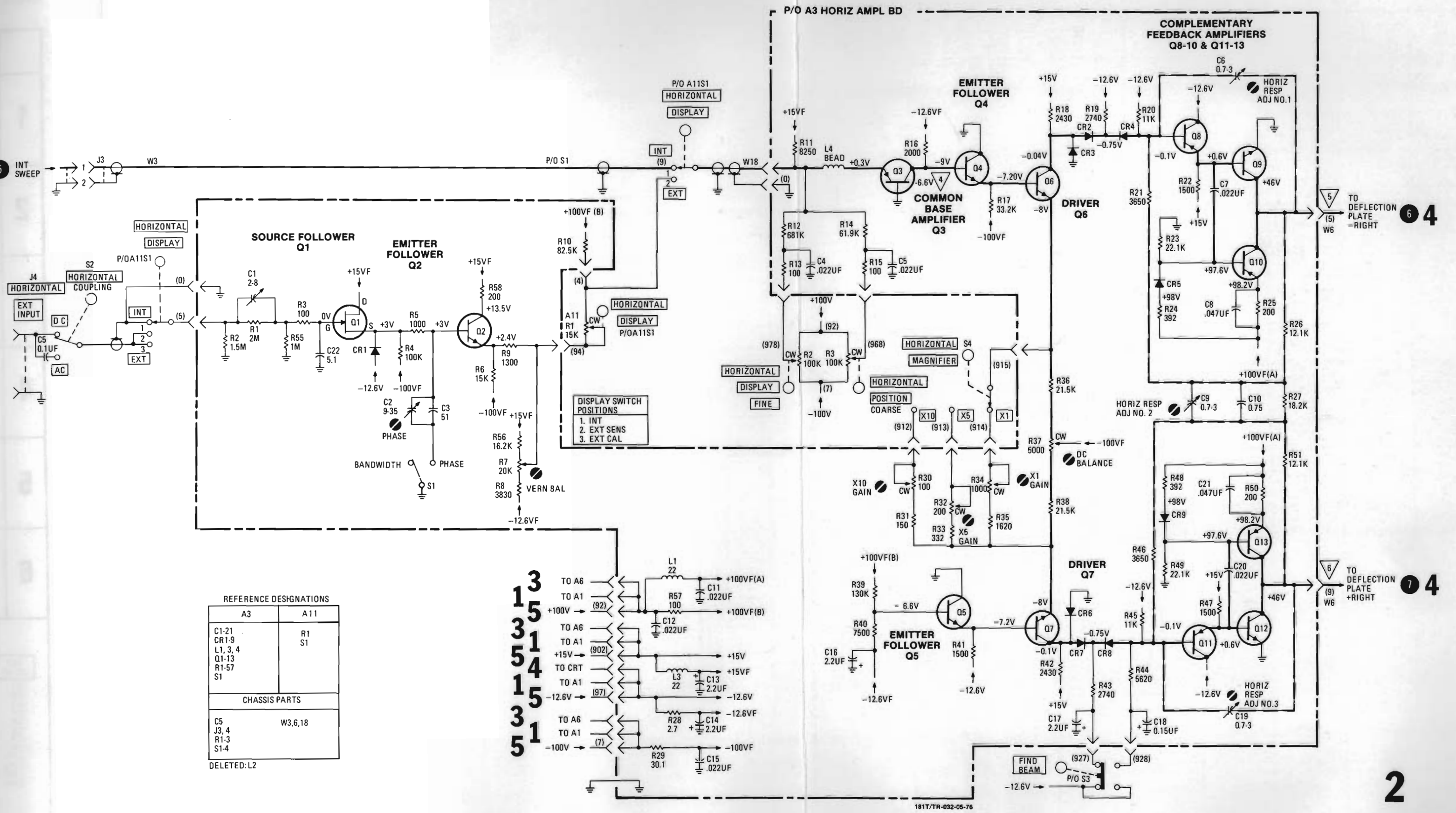
Figure 8-10. Horizontal Amplifier 8-13
