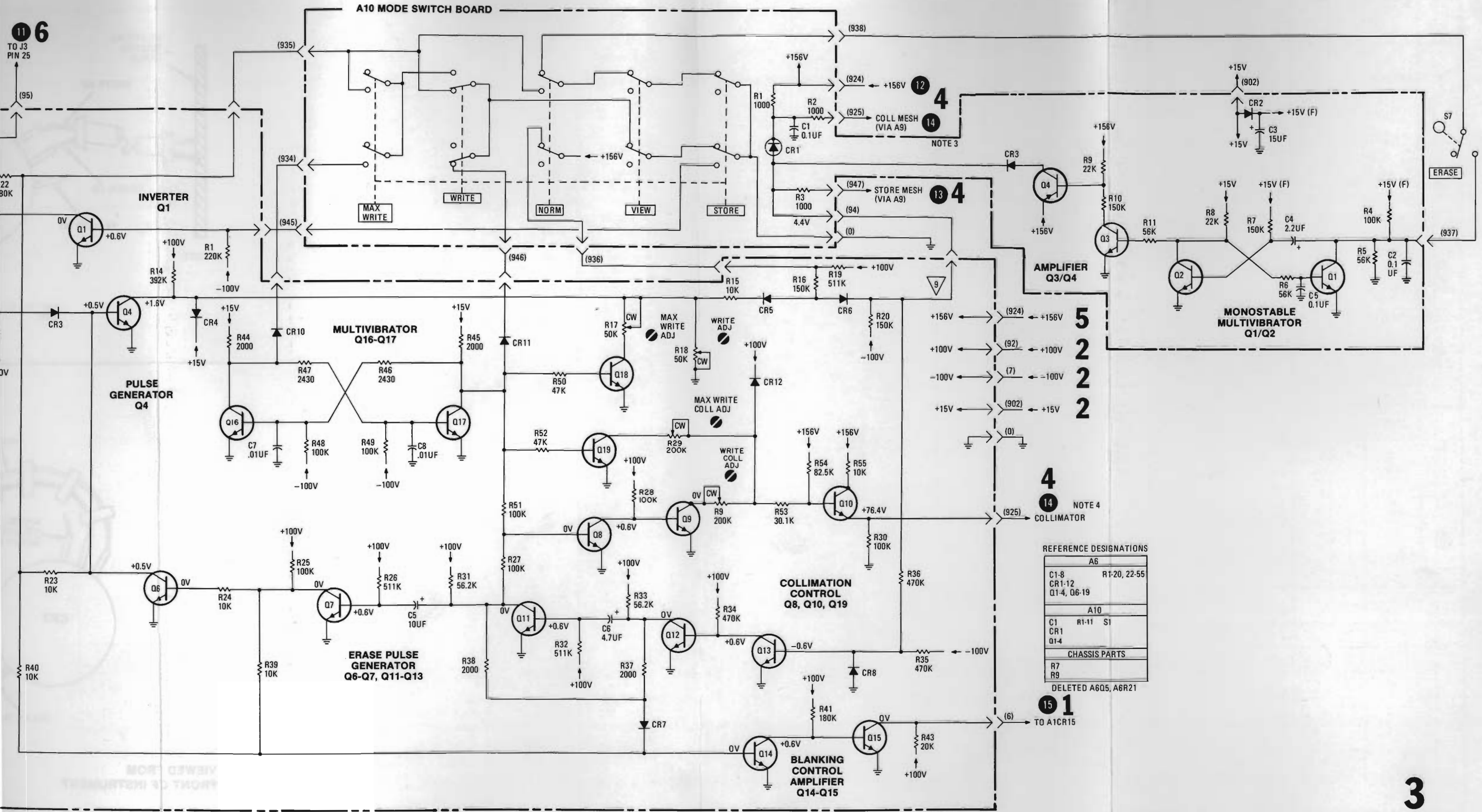
Figure 8-14. Pulse Circuit 8-15
