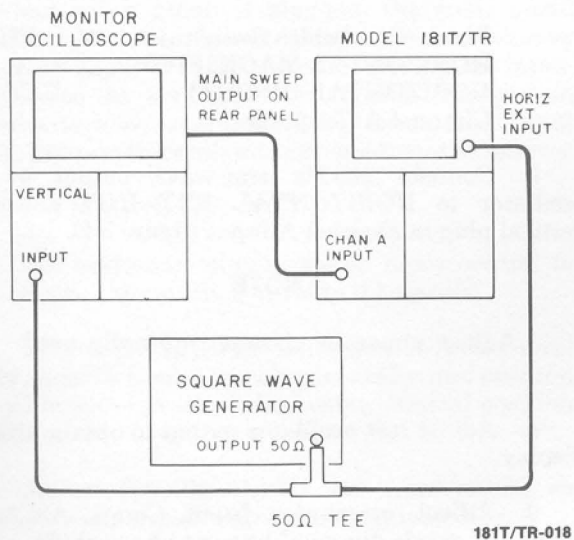
Figure 5-3. Transient Response Adj. Test Setup
