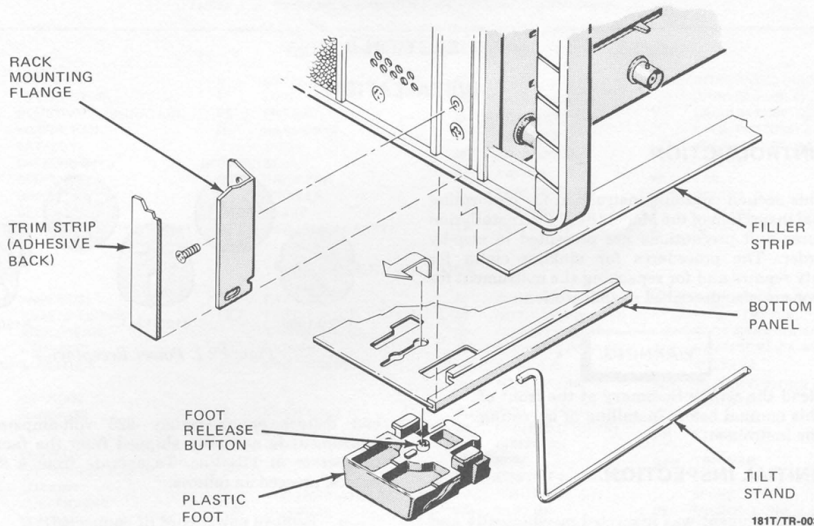
Figure 2-2. Bench/Rack-Mount Conversion
