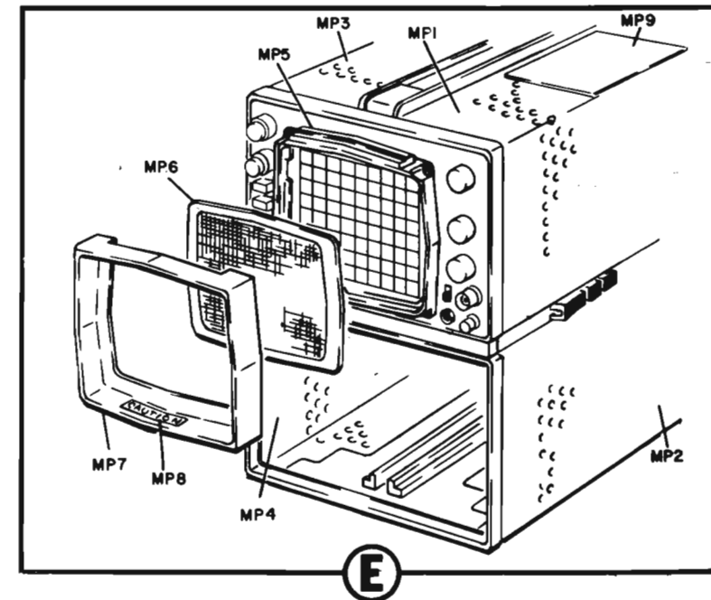
Figure 6-1. Model 181T/TR Mechanical Parts Identification
